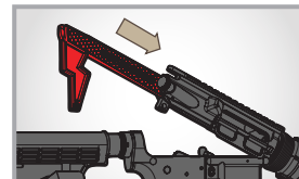
Remove bolt and insert the Smart Lock Bore Guide into the chamber
