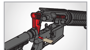
Snap pivot pin into place to hold the barrel in open position
