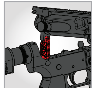
Pivot Lock holds gun open to optimal cleaning position
